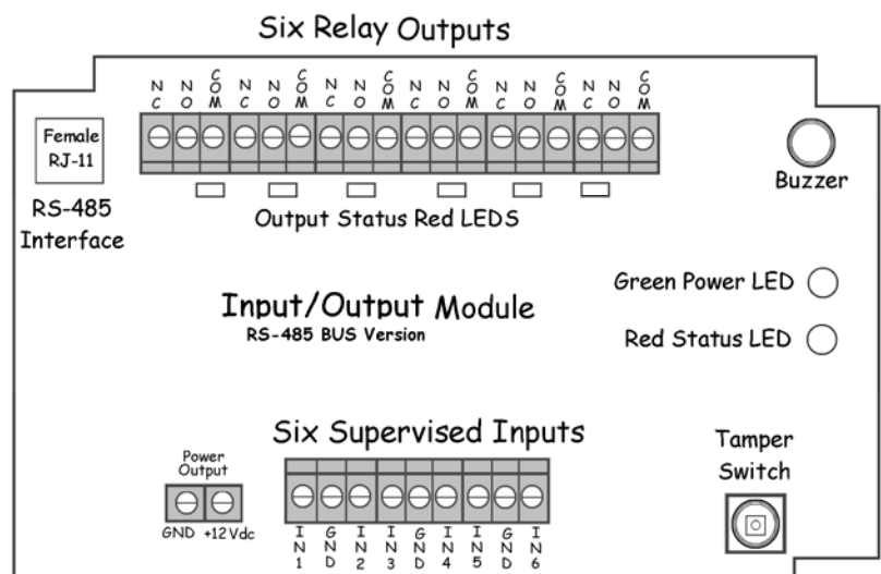
Elpas I/O Module (BUS Version) – Circuit Board
