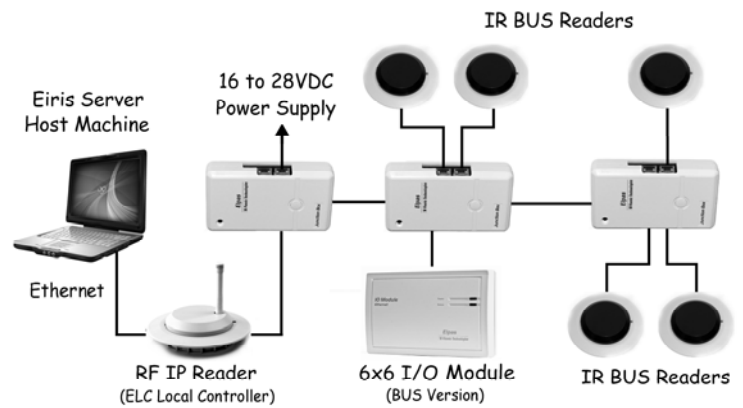
Elpas I/O Module (BUS Version) - Network Topology
