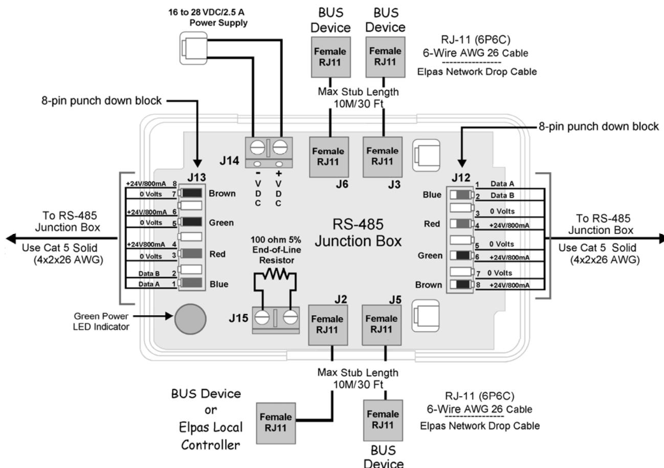
RS-485 Junction Module - Sample Wiring Topology
