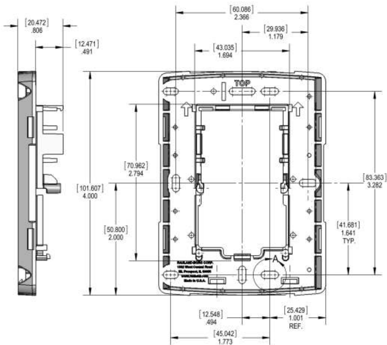
Figure 237: Responder® 4000 Slim Line Base Mounting Template
